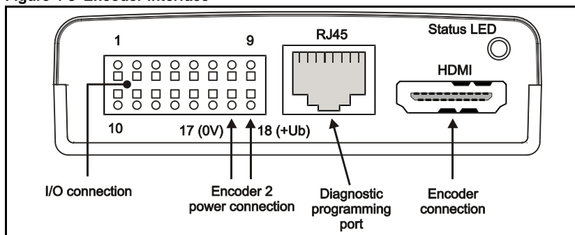
Figure 4-3 Encoder interface
